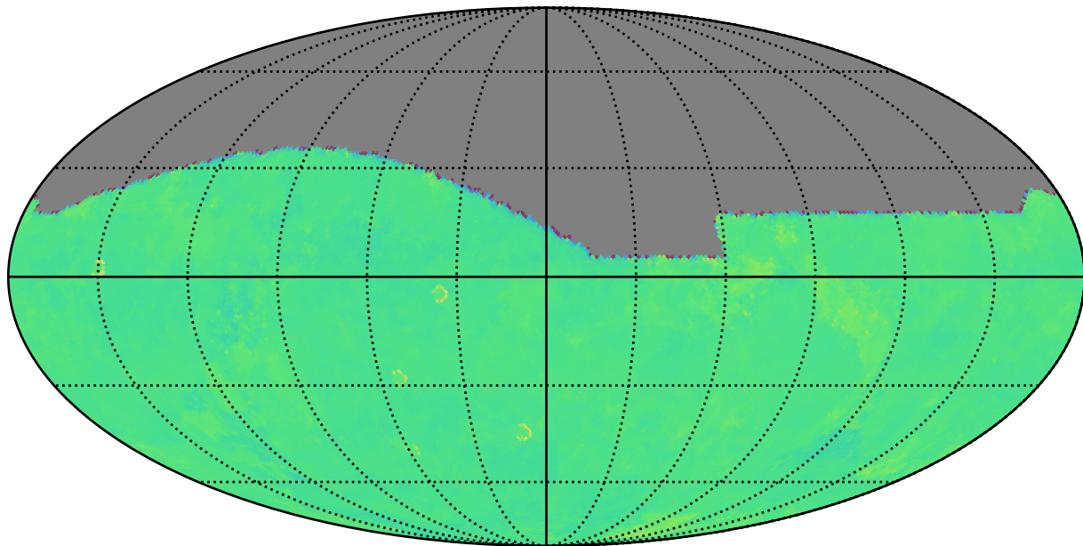
too_combined_s0.8_v3.4_10yrs g: Kuiper rotTelPos
