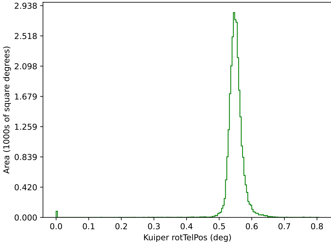
too_combined_s0.8_v3.4_10yrs g: Kuiper rotTelPos
