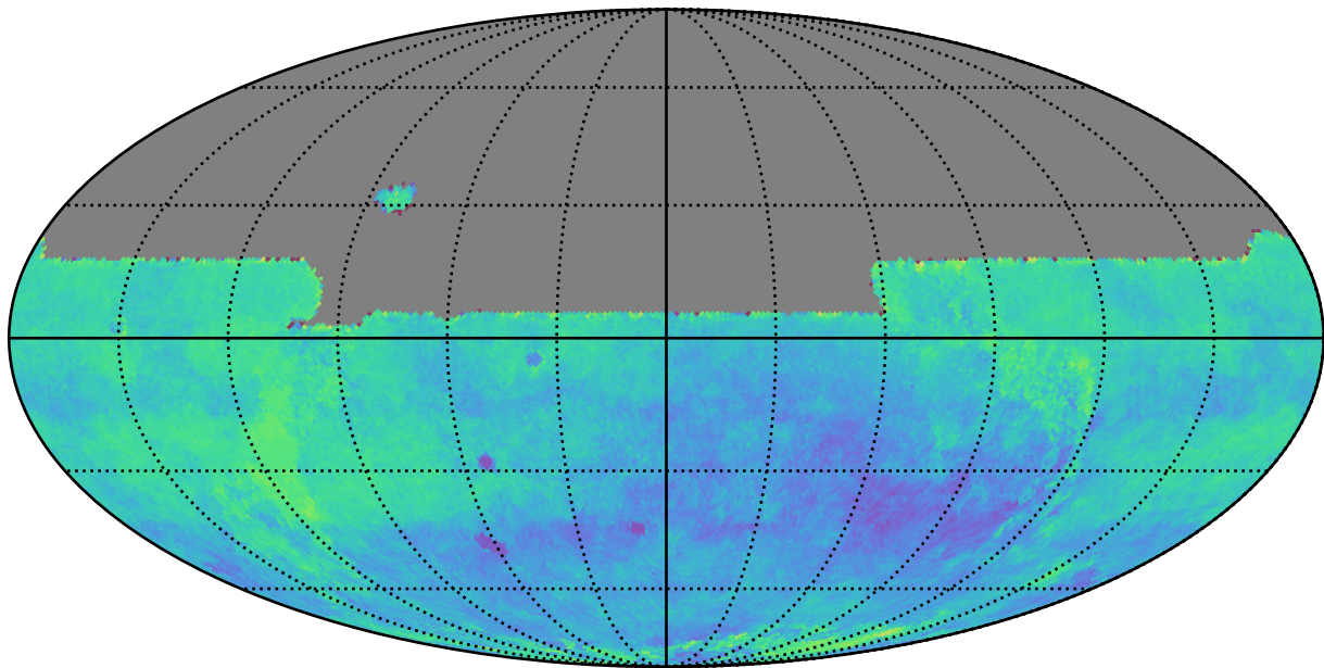
too_combined_s0.8_v3.4_10yrs y: Kuiper rotSkyPos
