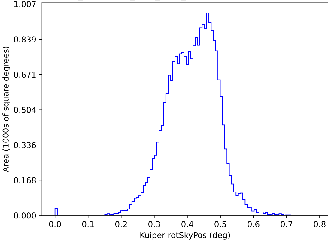
too_combined_s0.8_v3.4_10yrs y: Kuiper rotSkyPos
