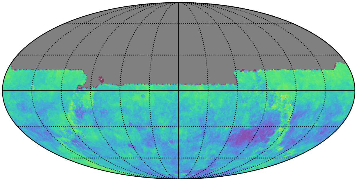
too_combined_s0.8_v3.4_10yrs u: Kuiper rotSkyPos
