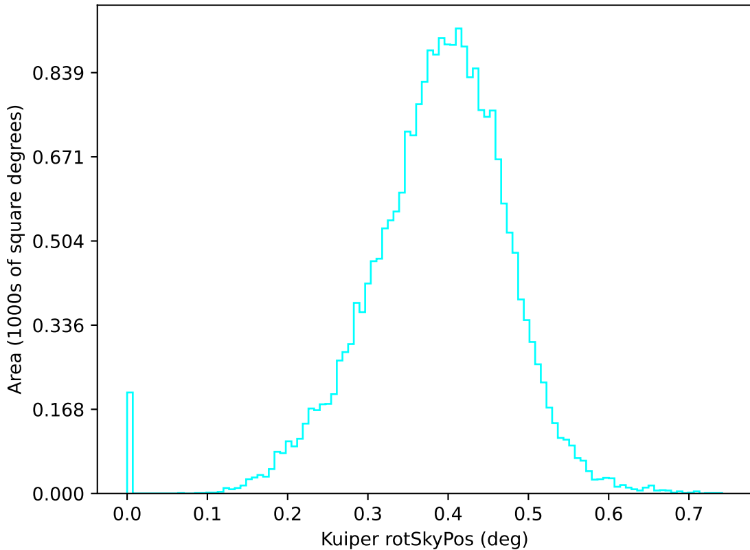
too_combined_s0.8_v3.4_10yrs u: Kuiper rotSkyPos
