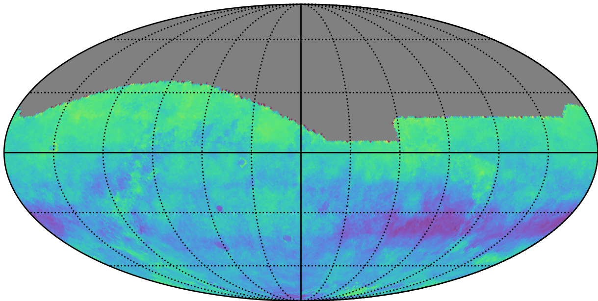
too_combined_s0.8_v3.4_10yrs r: Kuiper rotSkyPos
