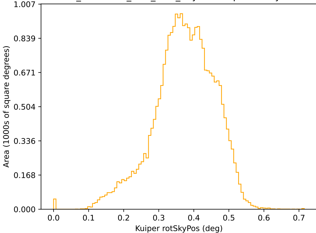
too_combined_s0.8_v3.4_10yrs r: Kuiper rotSkyPos
