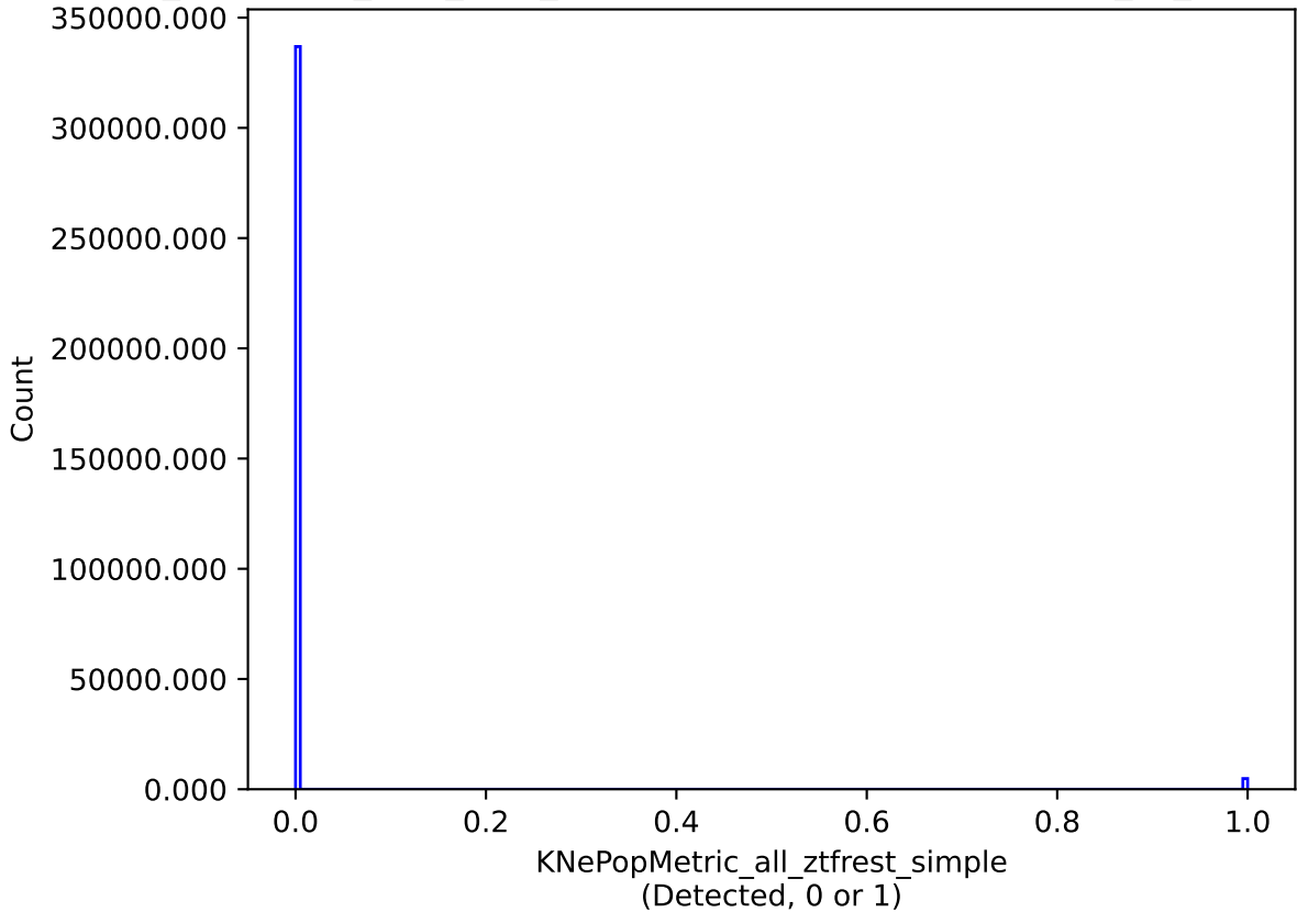
too_combined_s0.8_v3.4_10yrs all models: KNePopMetric_all_ztfrest_simple
