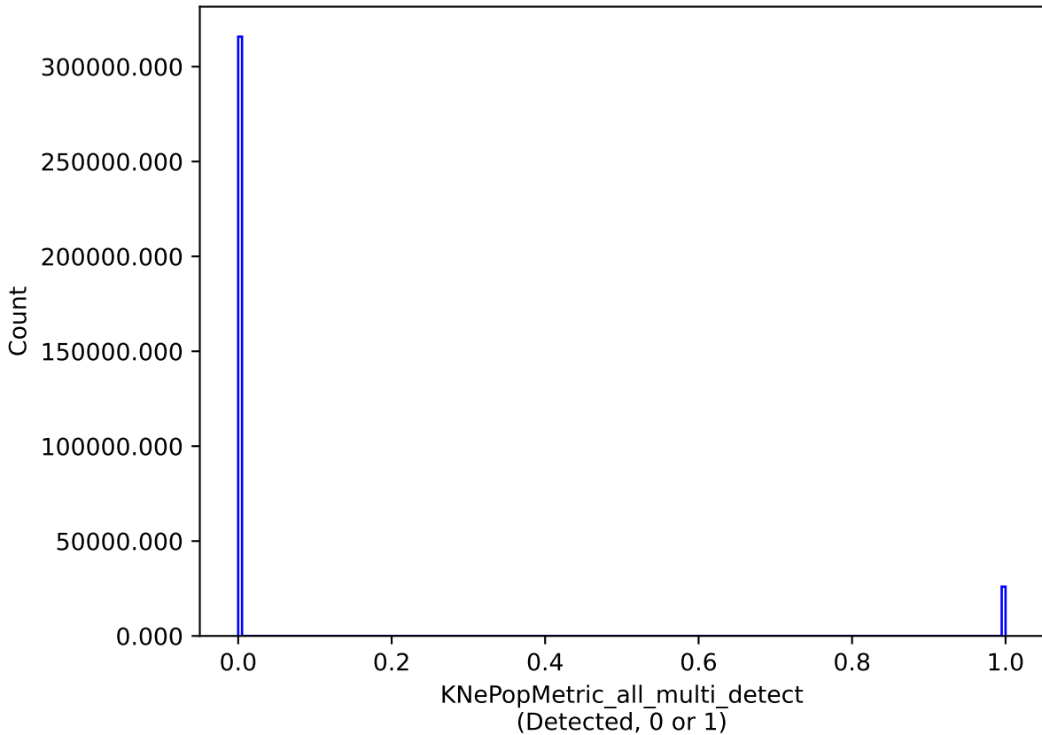
too_combined_s0.8_v3.4_10yrs all models: KNePopMetric_all_multi_detect
