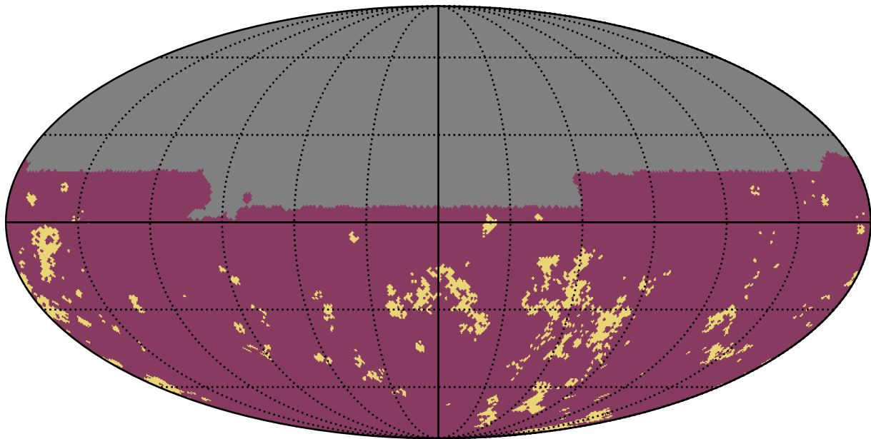
too_combined_s0.8_v3.4_10yrs u band: Gaps_7hr
