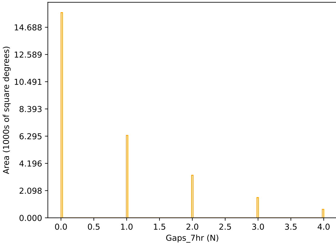
too_combined_s0.8_v3.4_10yrs r band: Gaps_7hr
