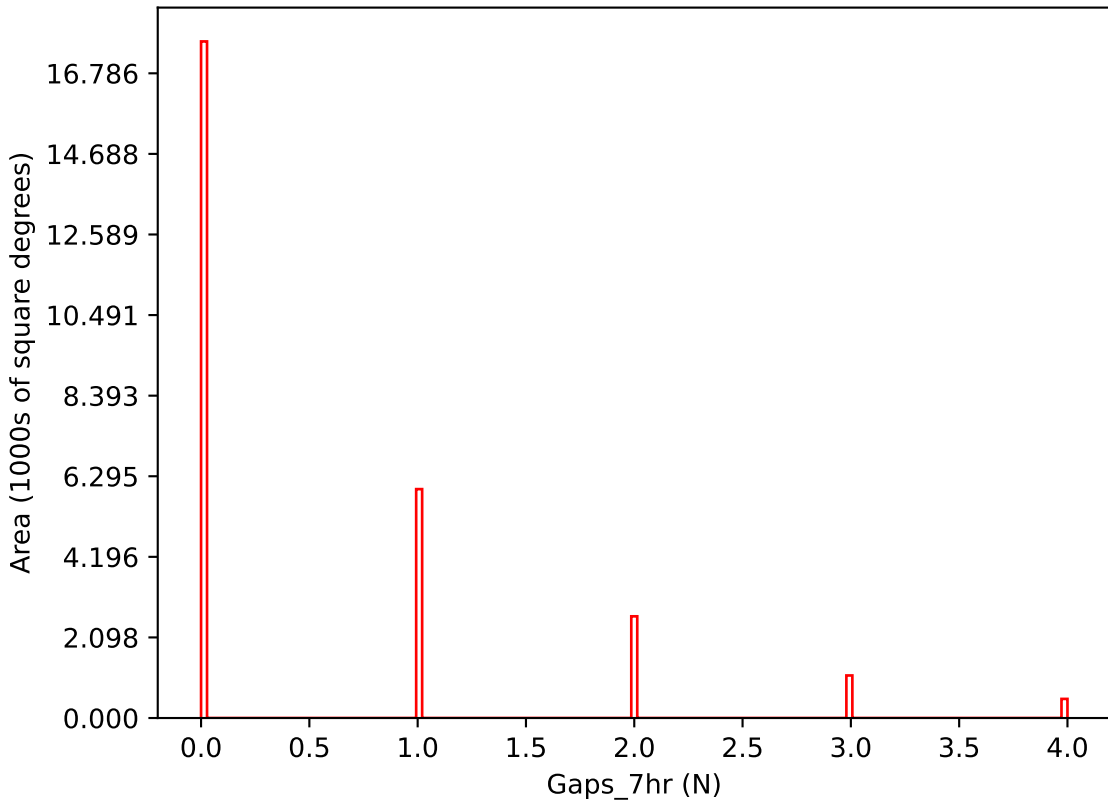
too_combined_s0.8_v3.4_10yrs i band: Gaps_7hr
