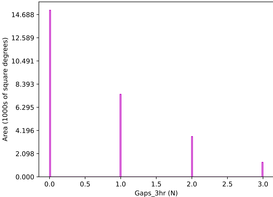
too_combined_s0.8_v3.4_10yrs z band: Gaps_3hr
