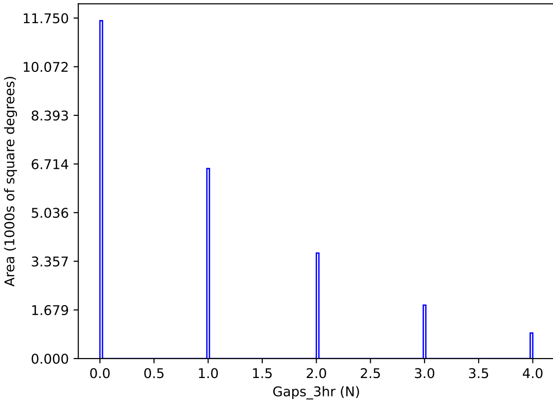
too_combined_s0.8_v3.4_10yrs y band: Gaps_3hr
