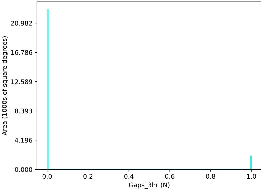
too_combined_s0.8_v3.4_10yrs u band: Gaps_3hr
