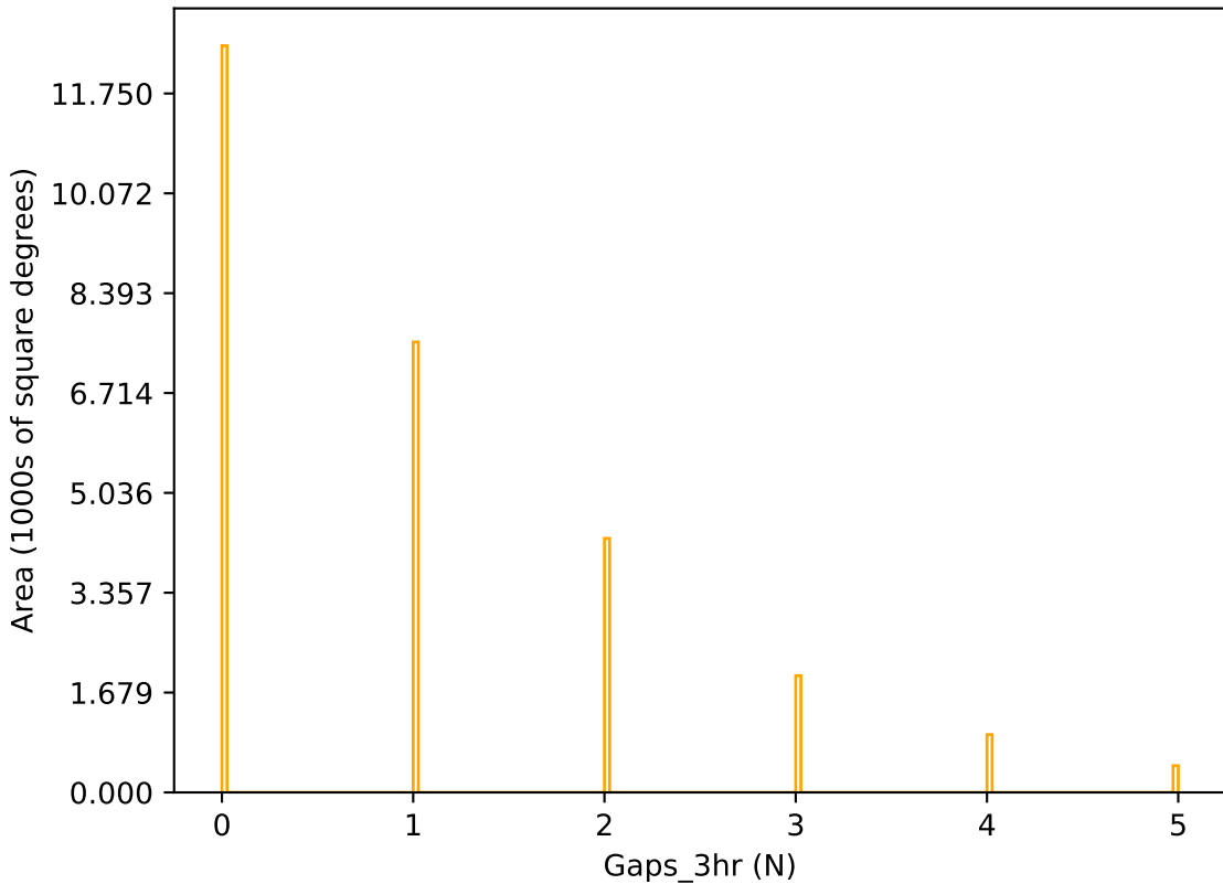
too_combined_s0.8_v3.4_10yrs r band: Gaps_3hr
