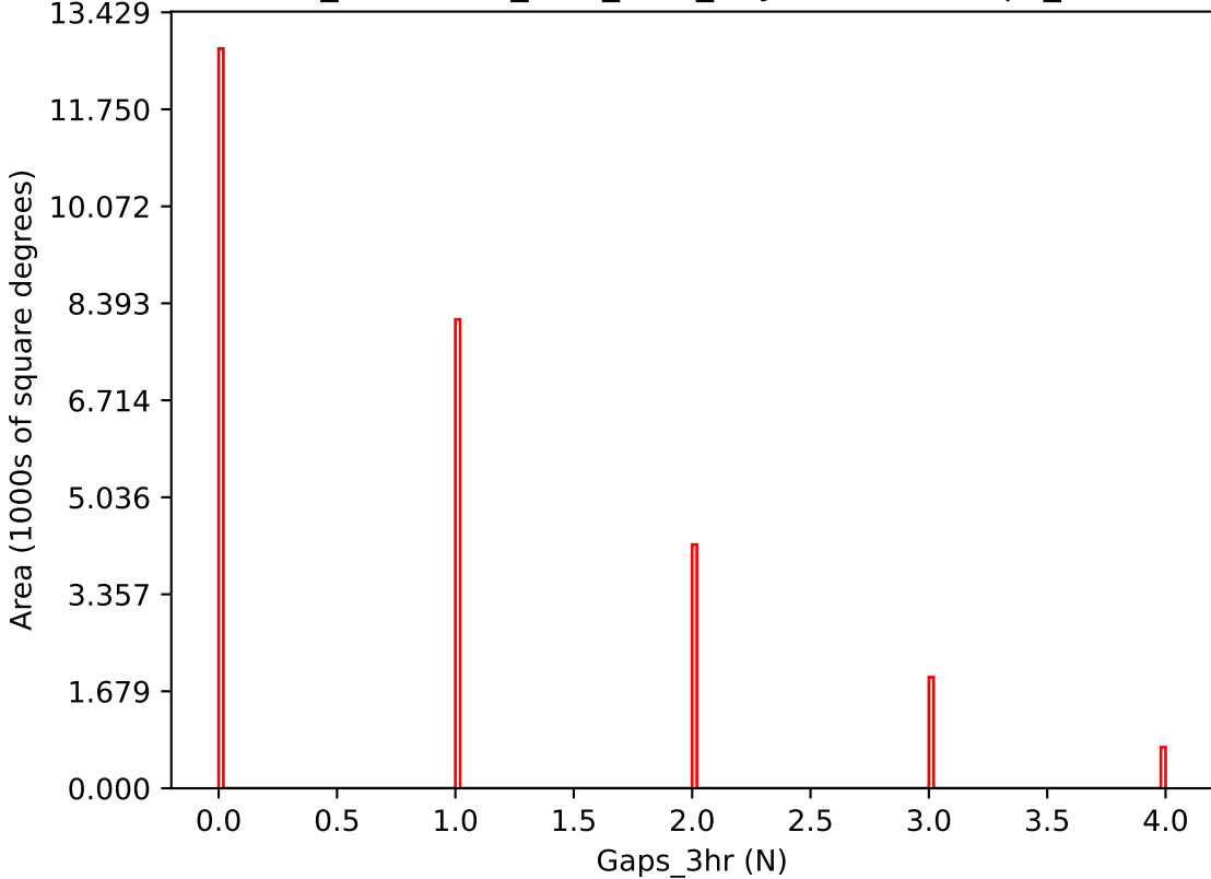
too_combined_s0.8_v3.4_10yrs i band: Gaps_3hr
