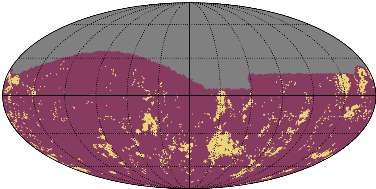
too_combined_s0.8_v3.4_10yrs g band: Gaps_3hr
