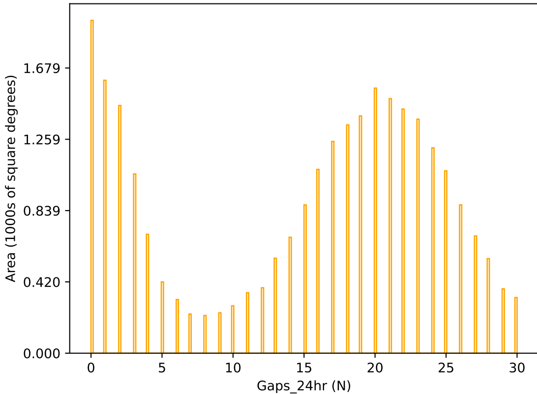
too_combined_s0.8_v3.4_10yrs r band: Gaps_24hr
