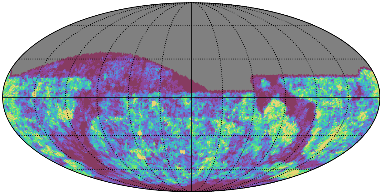
too_combined_s0.8_v3.4_10yrs g band: Gaps_24hr
