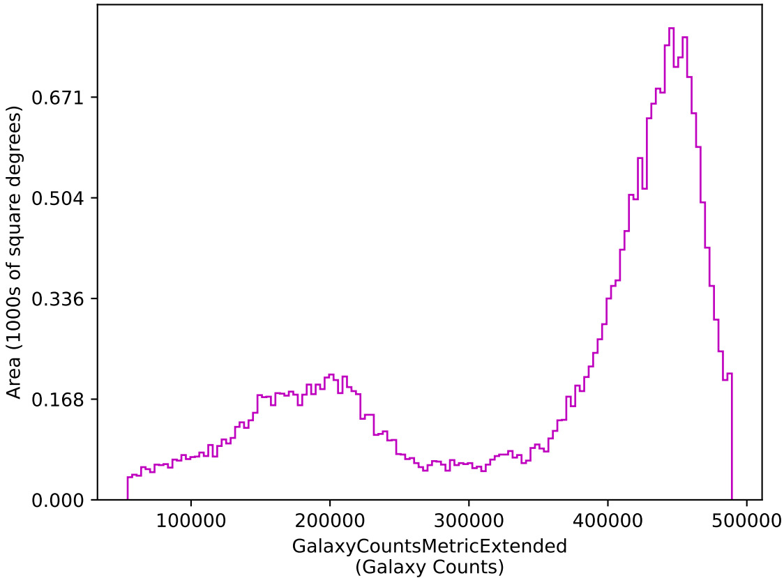
too_combined_s0.8_v3.4_10yrs z: GalaxyCountsMetricExtended
