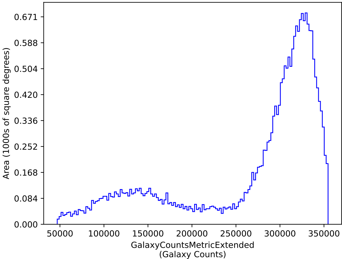
too_combined_s0.8_v3.4_10yrs y: GalaxyCountsMetricExtended
