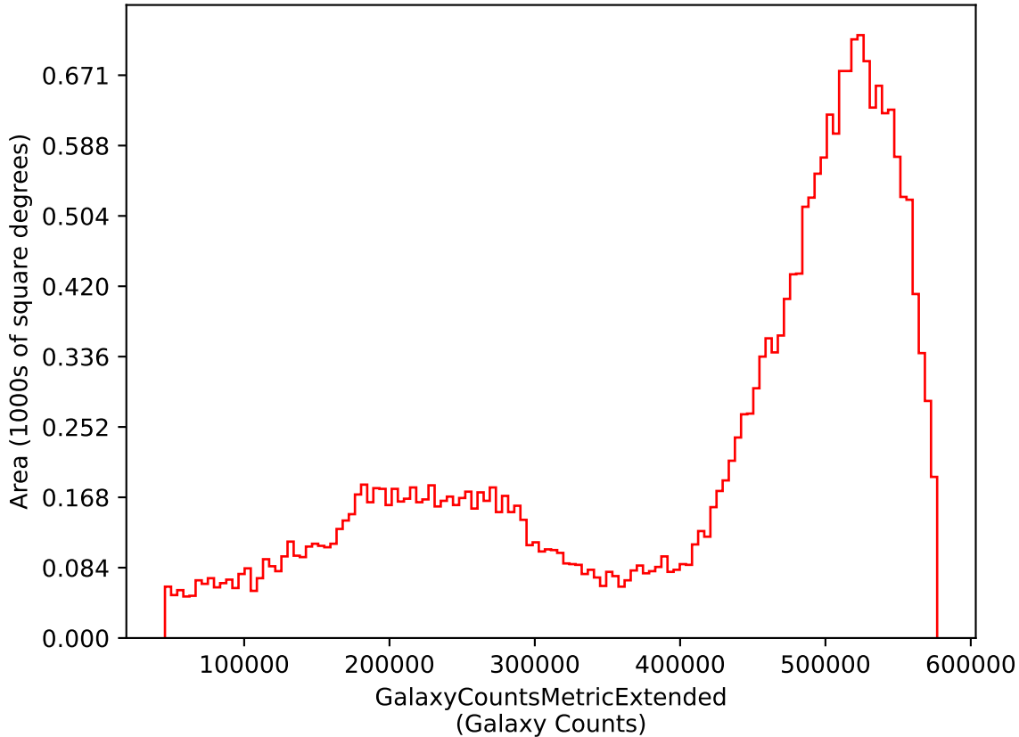
too_combined_s0.8_v3.4_10yrs i: GalaxyCountsMetricExtended
