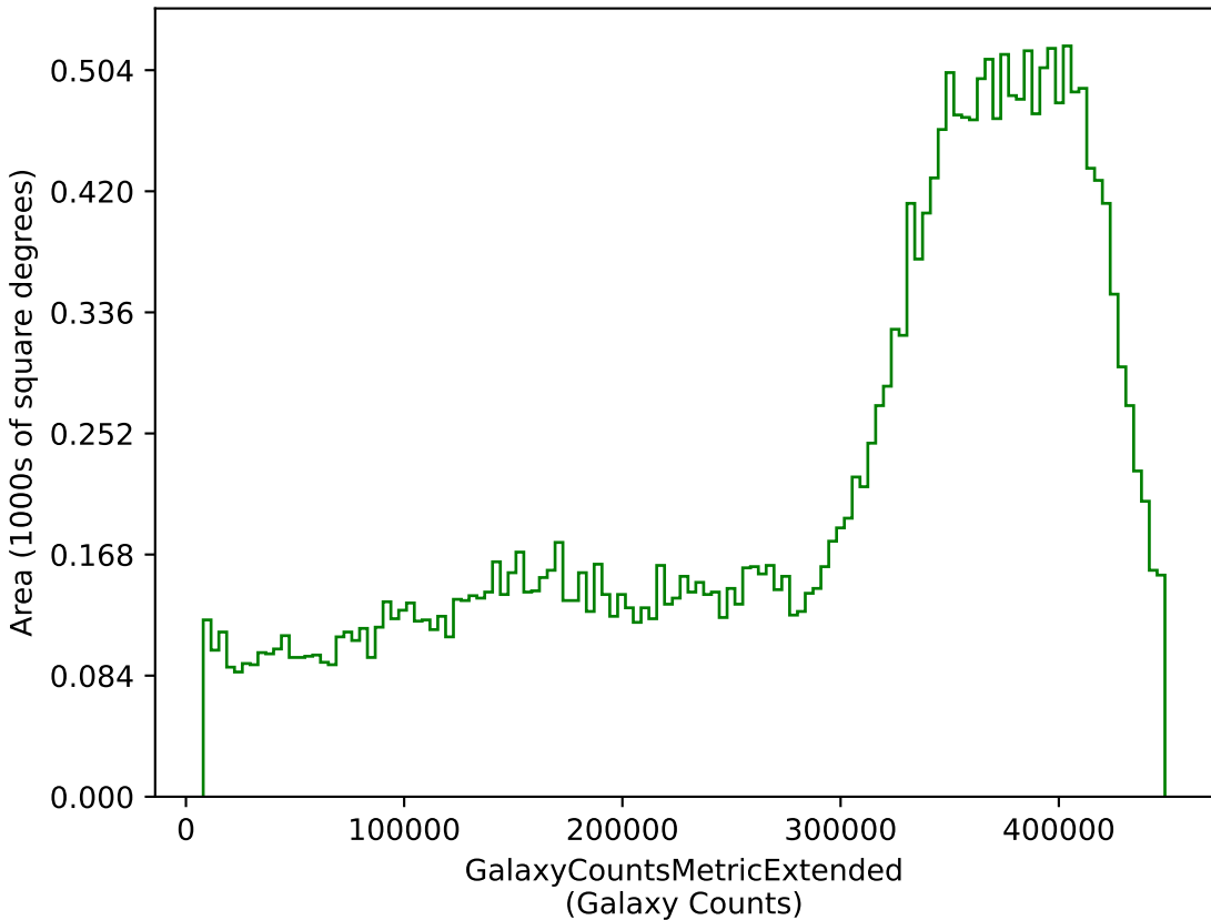
too_combined_s0.8_v3.4_10yrs g: GalaxyCountsMetricExtended
