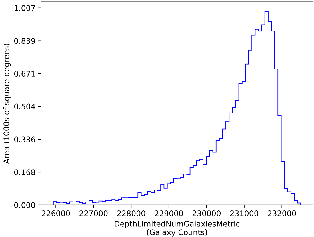
too_combined_s0.8_v3.4_10yrs i band galaxies non-DD: DepthLimitedNumGalaxiesMetric
