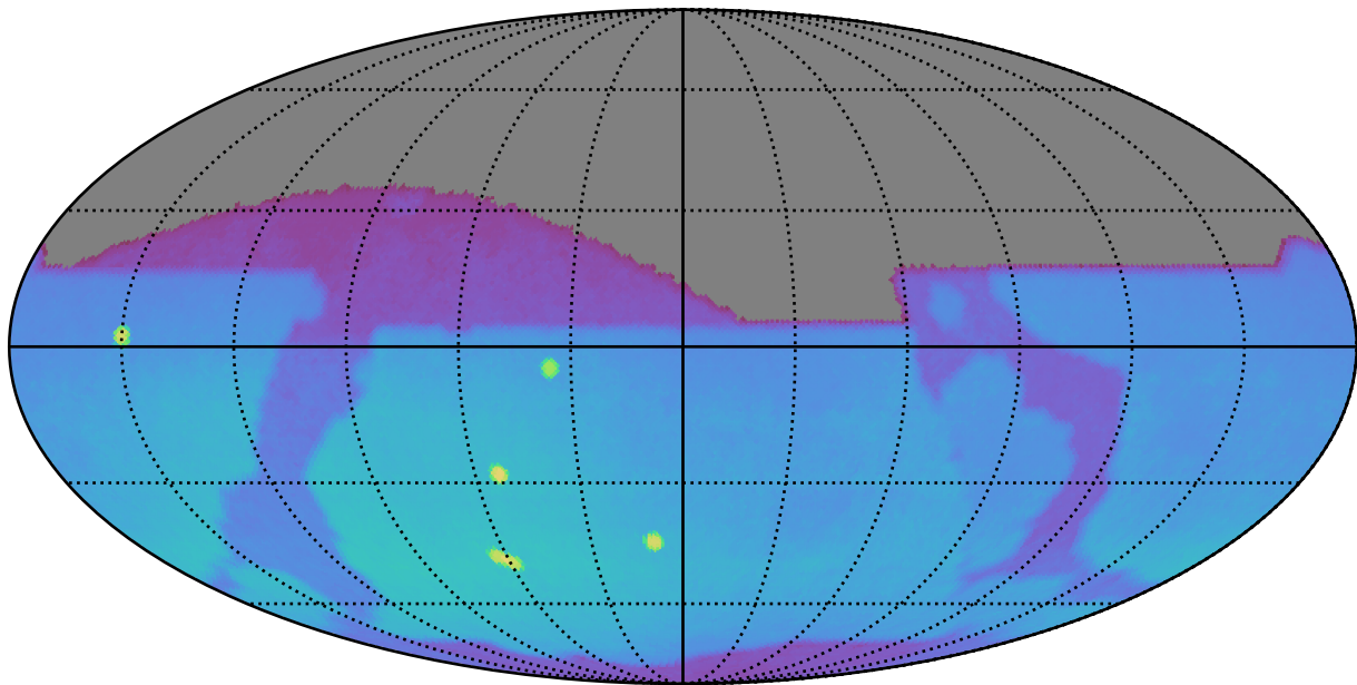
too_combined_s0.8_v3.4_10yrs : Brown Dwarf, L7
