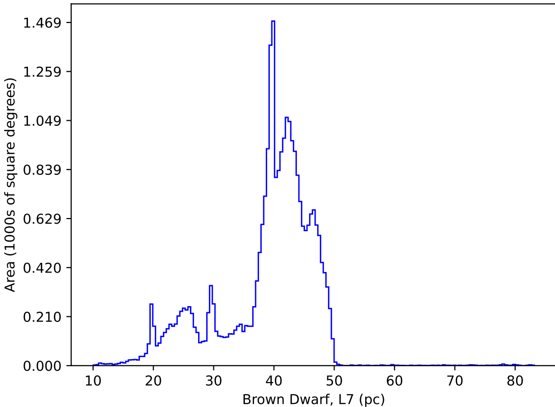
too_combined_s0.8_v3.4_10yrs : Brown Dwarf, L7
