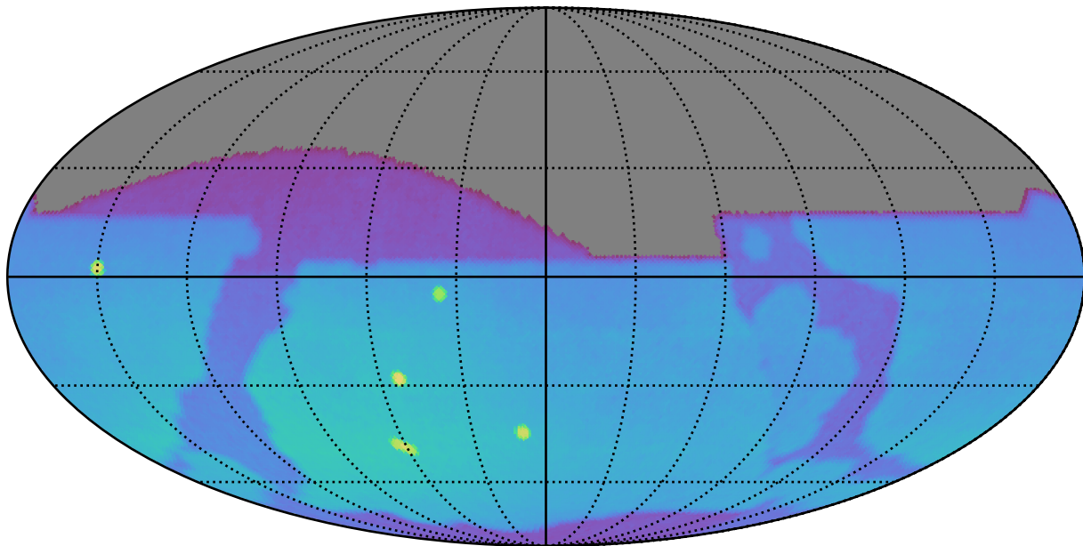
too_combined_s0.8_v3.4_10yrs : Brown Dwarf, L4
