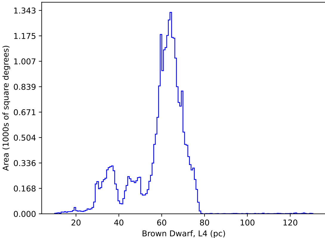
too_combined_s0.8_v3.4_10yrs : Brown Dwarf, L4
