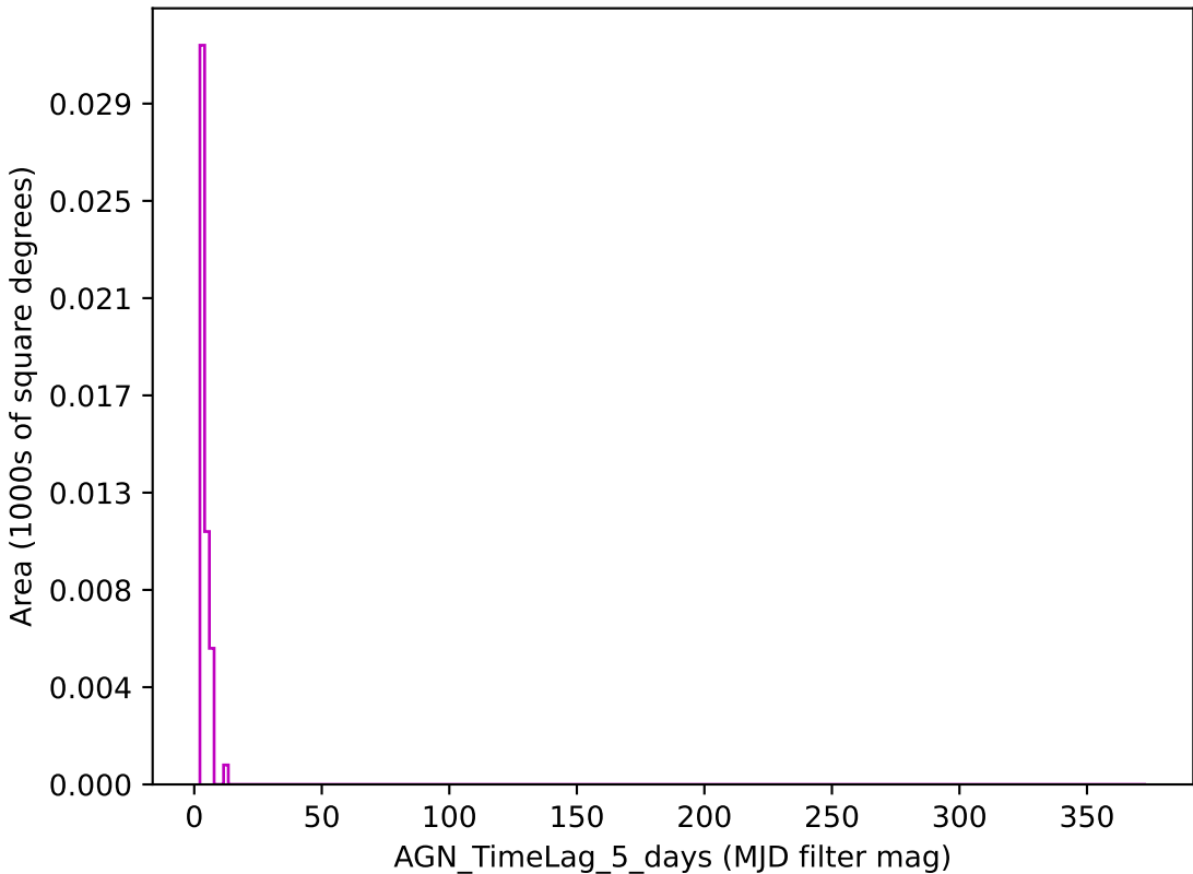
too_combined_s0.8_v3.4_10yrs z band: AGN_TimeLag_5_days
