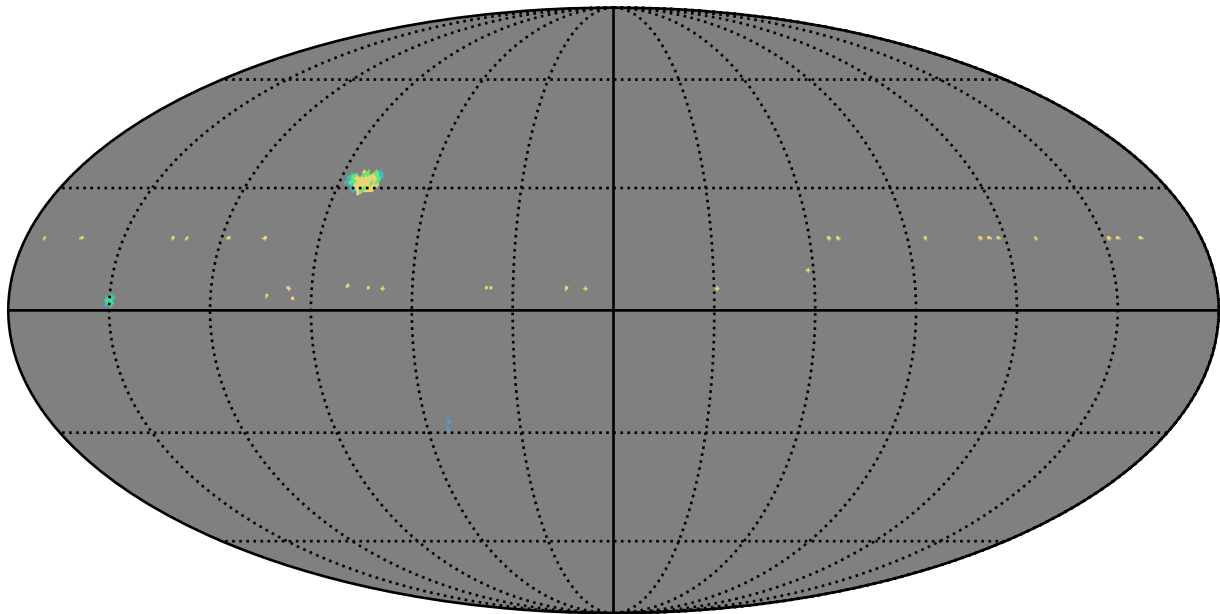
too_combined_s0.8_v3.4_10yrs y band: AGN_TimeLag_5_days
