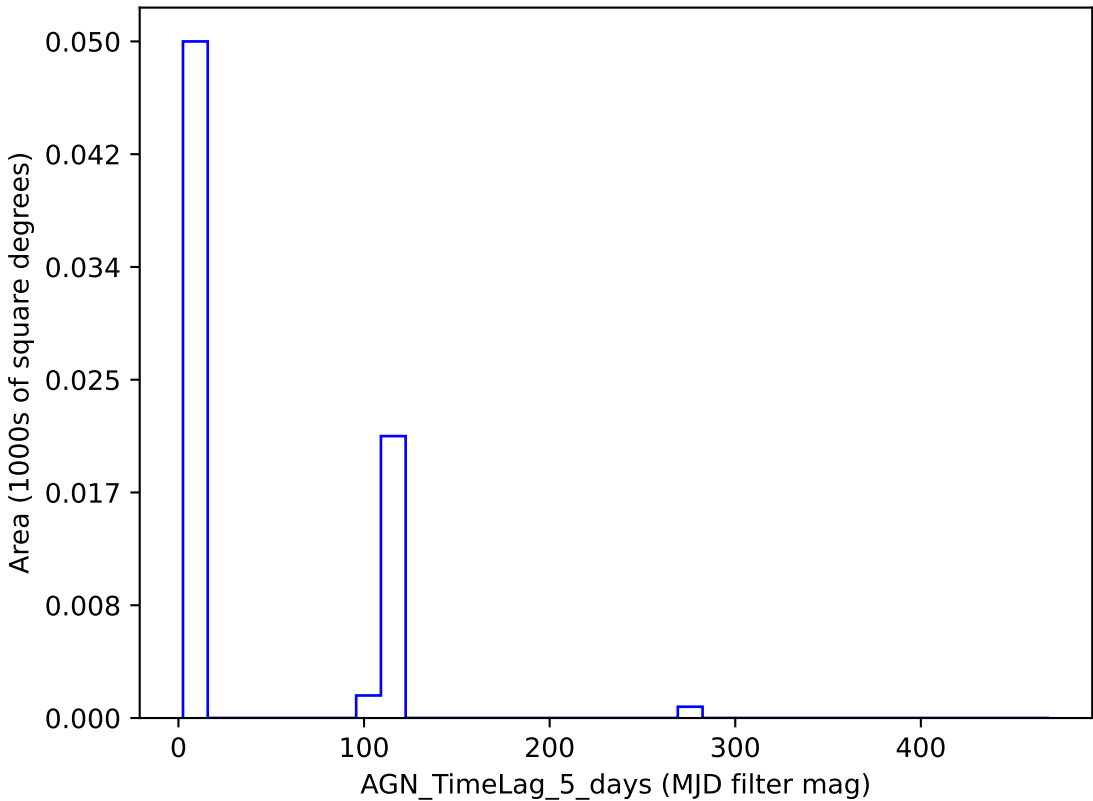
too_combined_s0.8_v3.4_10yrs y band: AGN_TimeLag_5_days
