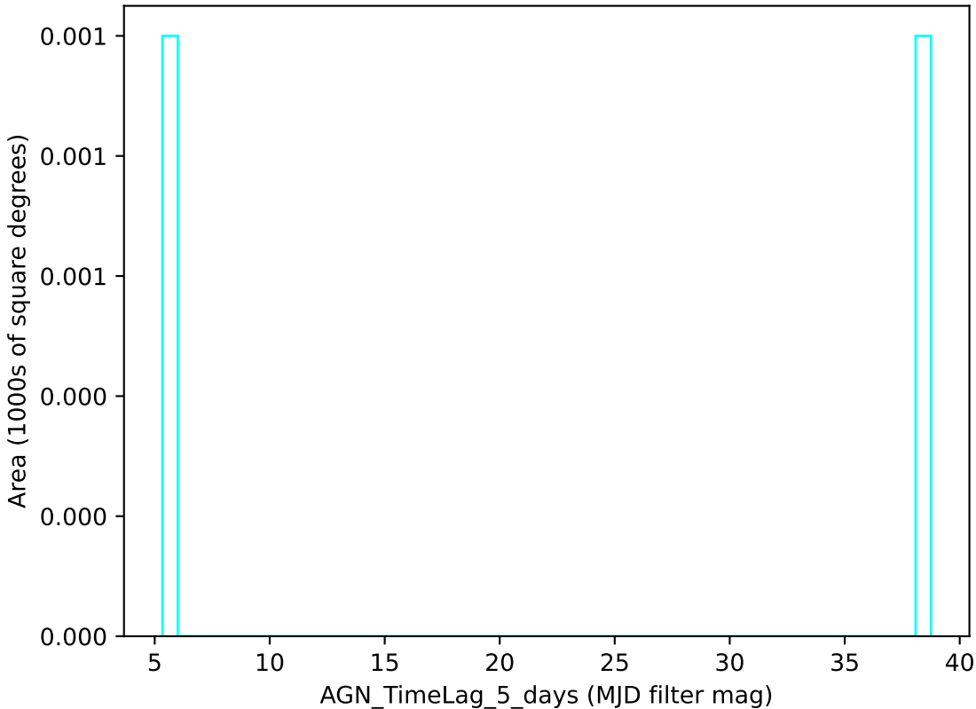
too_combined_s0.8_v3.4_10yrs u band: AGN_TimeLag_5_days
