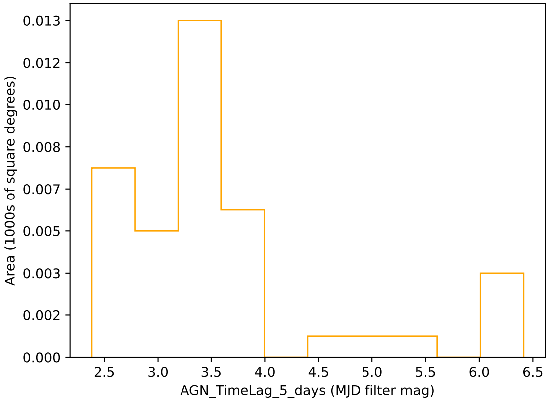
too_combined_s0.8_v3.4_10yrs r band: AGN_TimeLag_5_days
