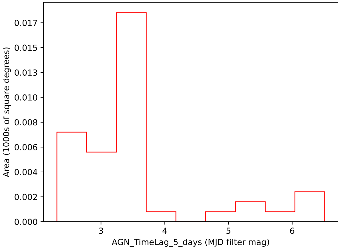
too_combined_s0.8_v3.4_10yrs i band: AGN_TimeLag_5_days
