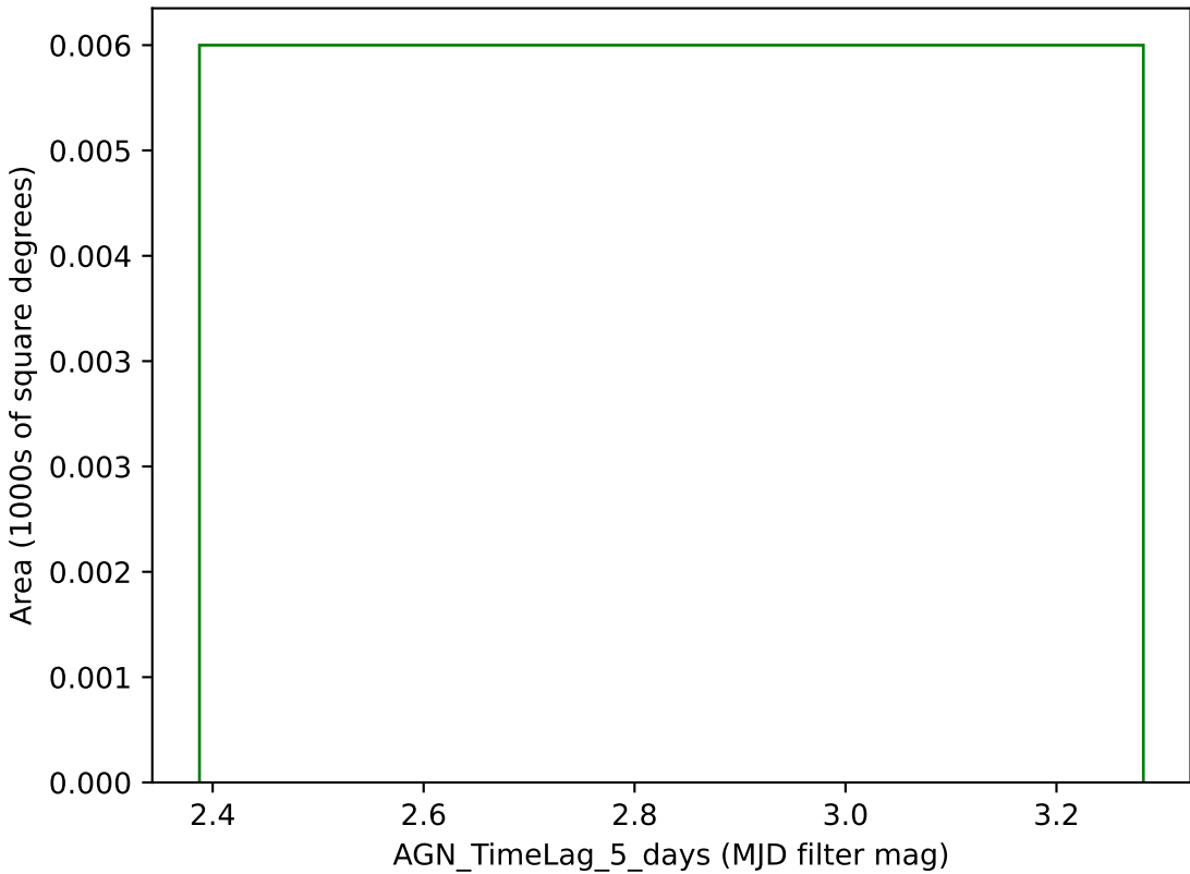
too_combined_s0.8_v3.4_10yrs g band: AGN_TimeLag_5_days
