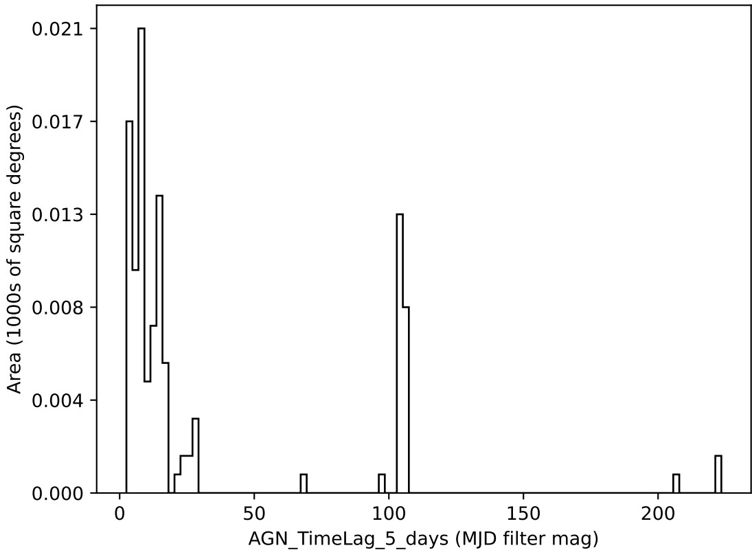
too_combined_s0.8_v3.4_10yrs all bands: AGN_TimeLag_5_days
