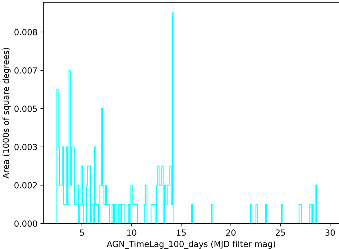
too_combined_s0.8_v3.4_10yrs u band: AGN_TimeLag_100_days
