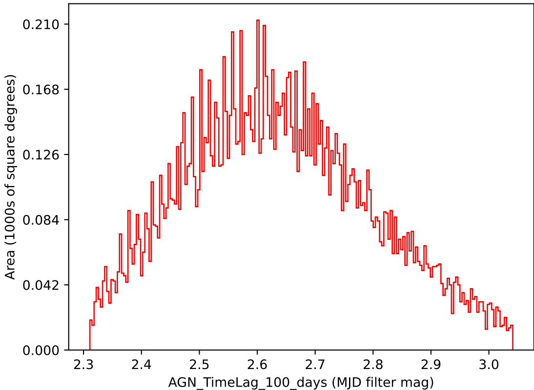
too_combined_s0.8_v3.4_10yrs i band: AGN_TimeLag_100_days
