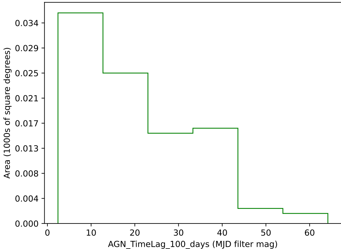
too_combined_s0.8_v3.4_10yrs g band: AGN_TimeLag_100_days
