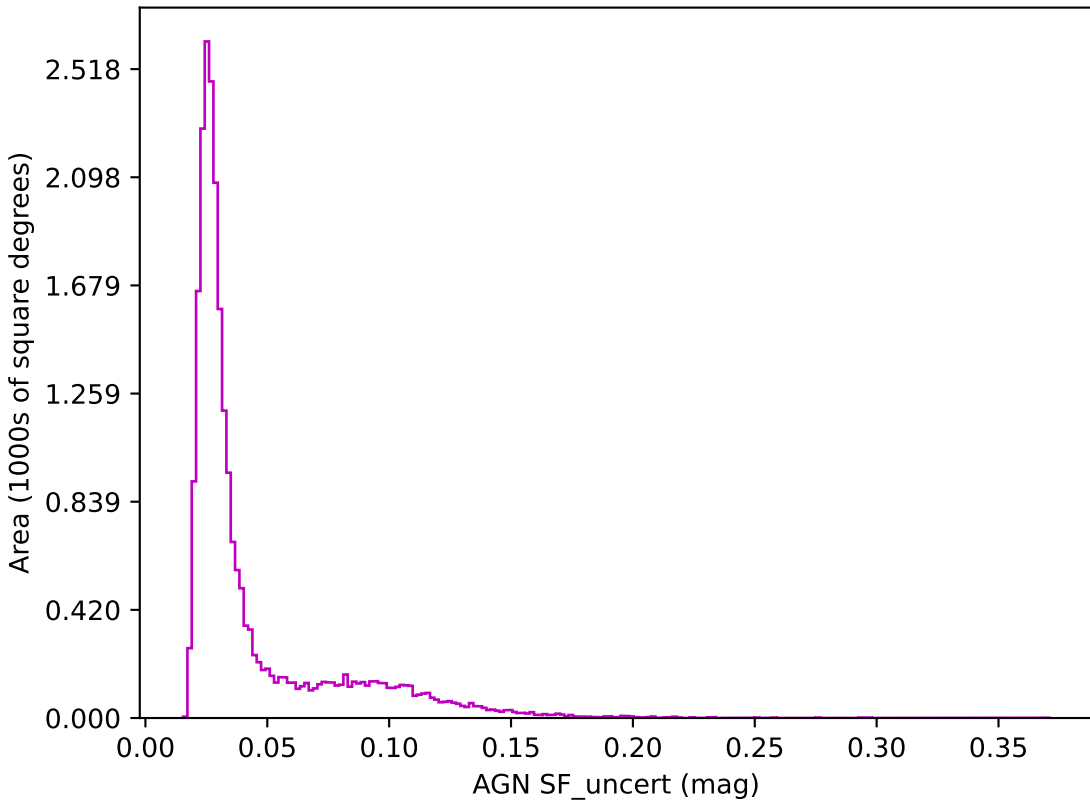
too_combined_s0.8_v3.4_10yrs z band: AGN SF_uncert
