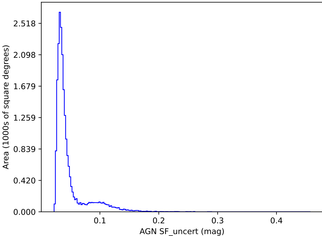
too_combined_s0.8_v3.4_10yrs y band: AGN SF_uncert
