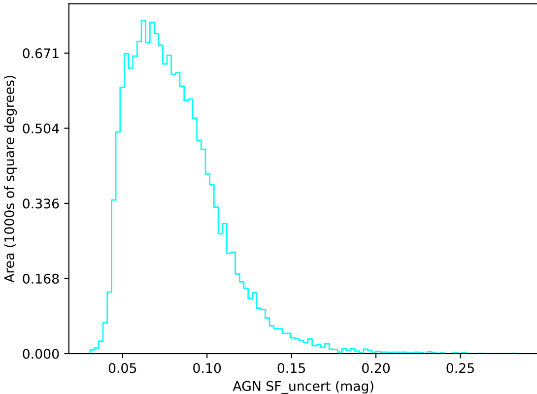
too_combined_s0.8_v3.4_10yrs u band: AGN SF_uncert
