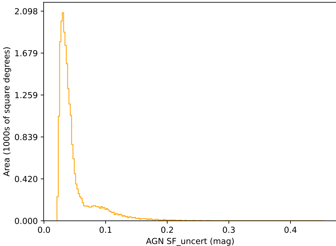
too_combined_s0.8_v3.4_10yrs r band: AGN SF_uncert
