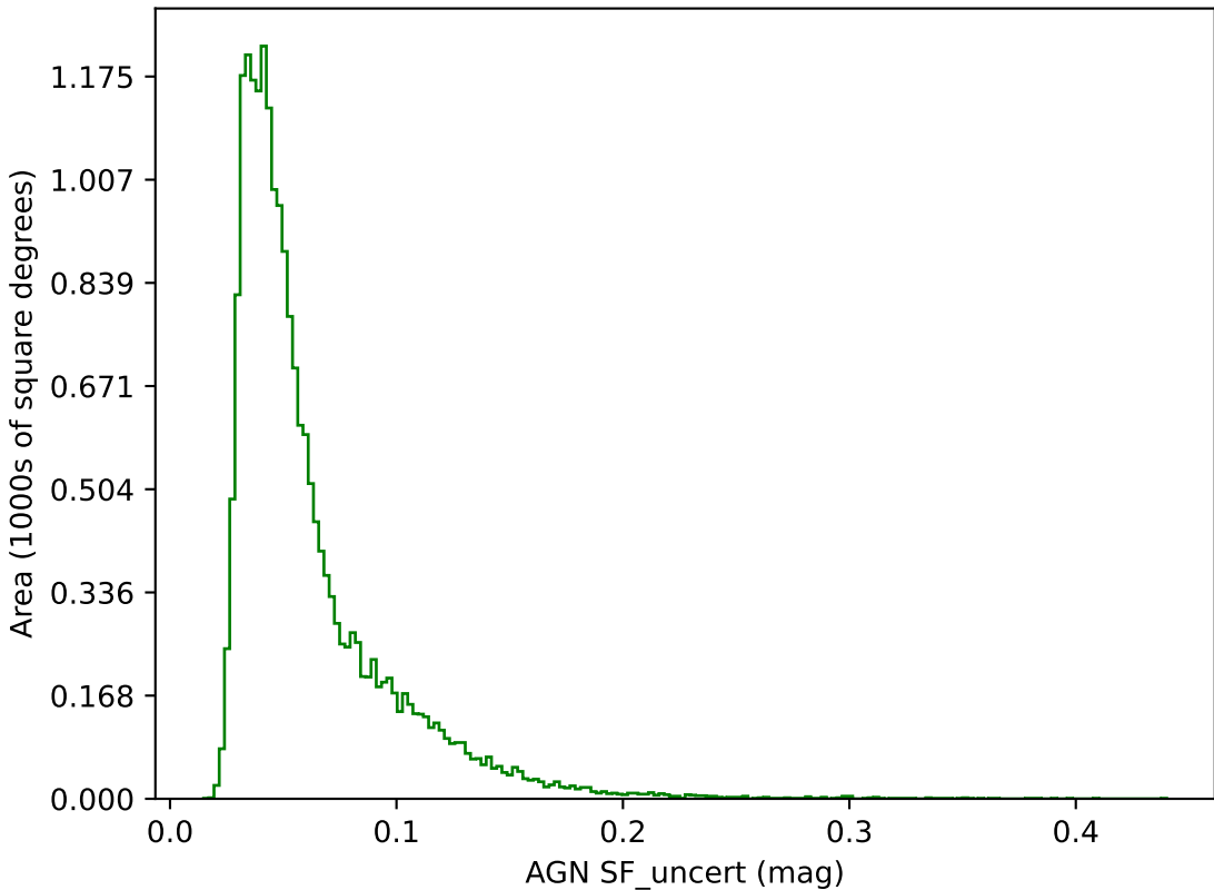
too_combined_s0.8_v3.4_10yrs g band: AGN SF_uncert
