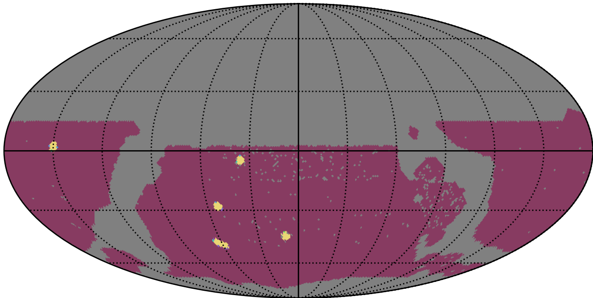
too_combined_s0.8_v3.4_10yrs WFD: NumberOfQuickRevisits
