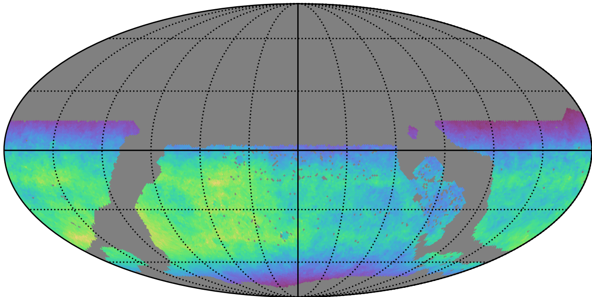
too_combined_s0.8_v3.4_10yrs WFD y band: Normalized Teff
