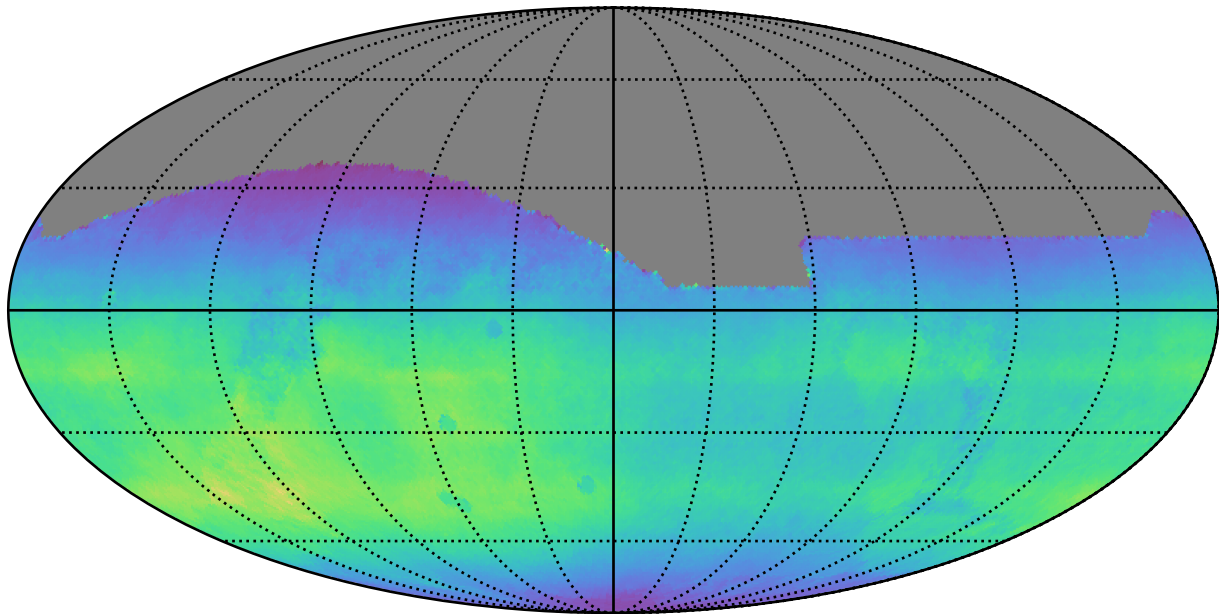
too_combined_s0.8_v3.4_10yrs All sky all bands: Normalized Teff
