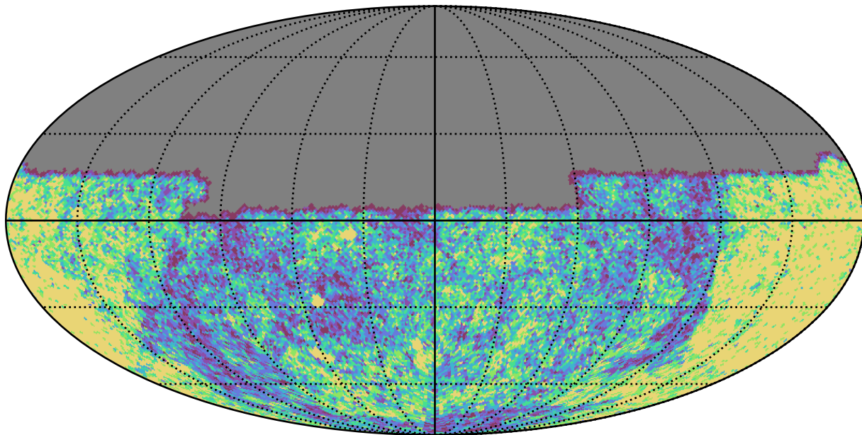
too_combined_s0.8_v3.4_10yrs Yr 1 u band: NVisits
